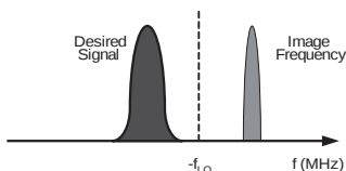
Figure 4. Image Frequency
