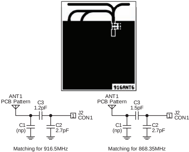
Figure 8. Example of a Multi-Element PCB
