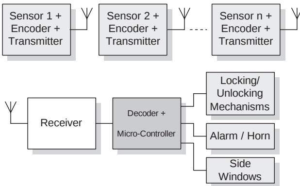
Figure 13. Remote Keyless Entry Application
