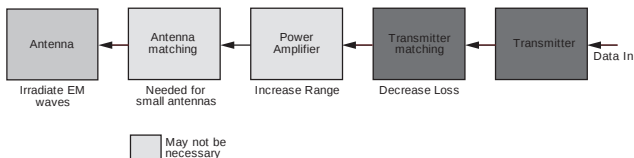
Figure 10. Transmitter Block Diagram
