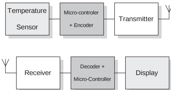
Figure 15. Telemetry Application
