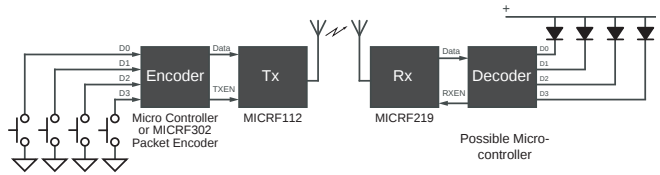
Figure 9. Block Diagram of a Wireless Application
