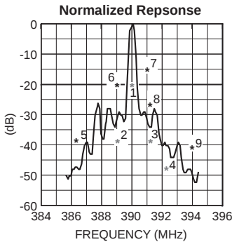
Figure 3. Effect of Interfering Signals on Sensitivity
