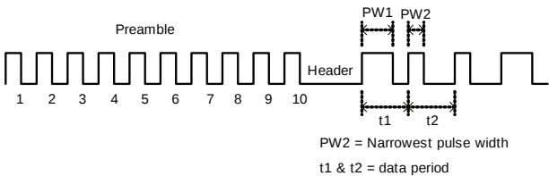
Figure 12. Suggest Data Pattern
