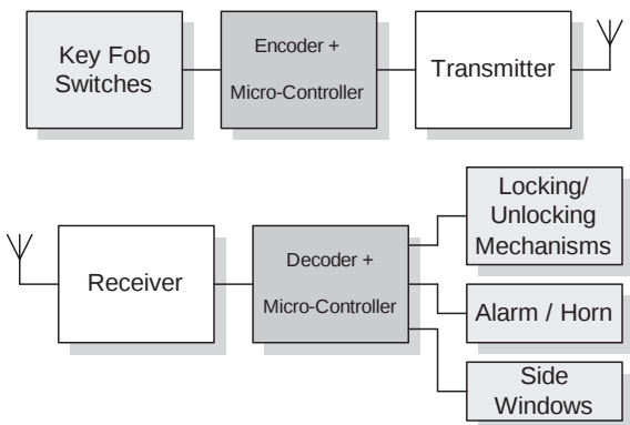
Figure 14. Alarm Application
