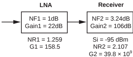
Figure 2. Improving Sensitivity by Adding a LNA
