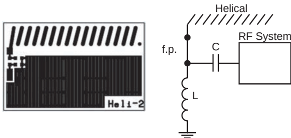
Figure 7. Example of a Helical PCB
