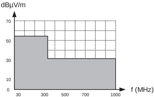
Figure 16. Power Levels for Japanese Regulation
