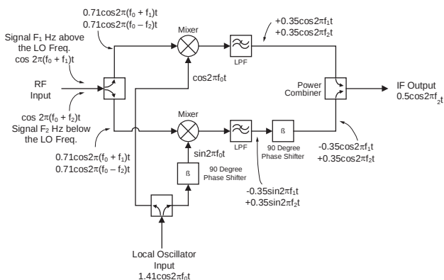
Figure 5. Image Reject Mixer
