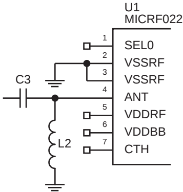
Figure 6. Suggested Matching Circuit
