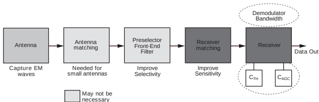
Figure 11. Receiver Block Diagram
