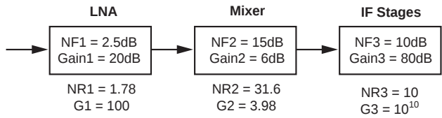
Figure 1. Stages of Noise for RF System
