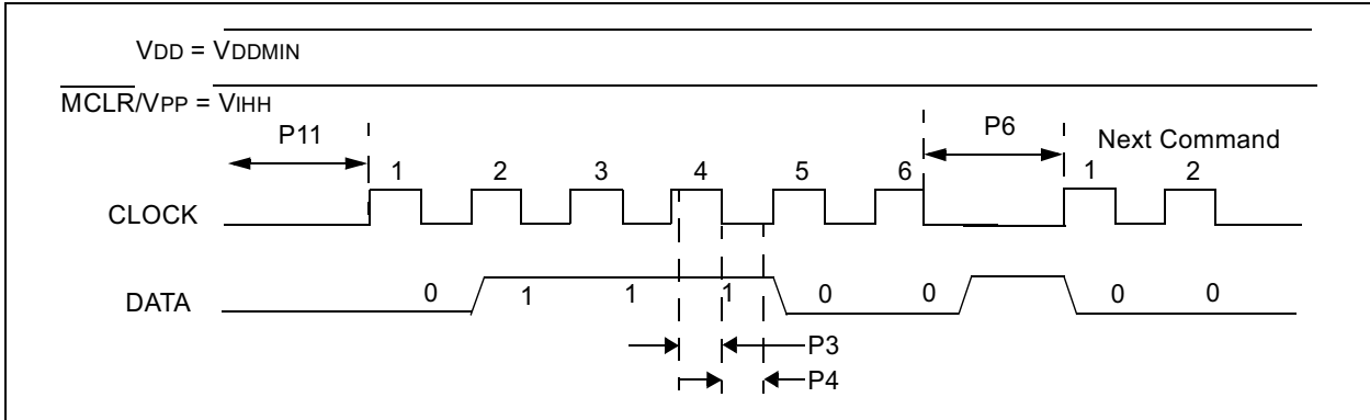
FIGURE 7-8: END PROGRAMMING COMMAND WAVEFORM
