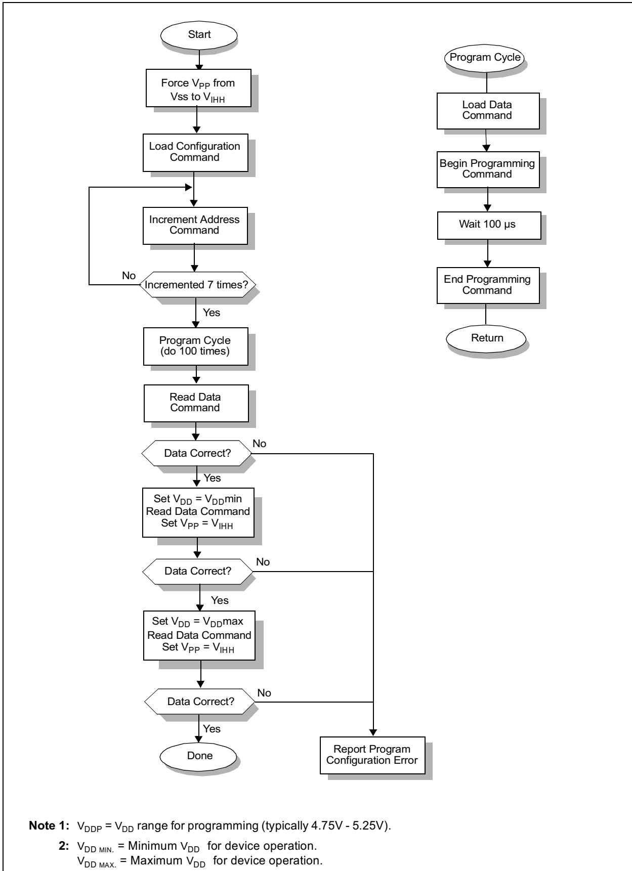
FIGURE 4-2: PROGRAM FLOW CHART - MCP250XX CONFIGURATION WORD
