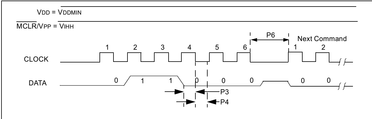
FIGURE 7-6: INCREMENT ADDRESS COMMAND WAVEFORM
